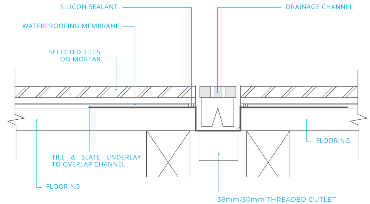
DETAIL VIEW
