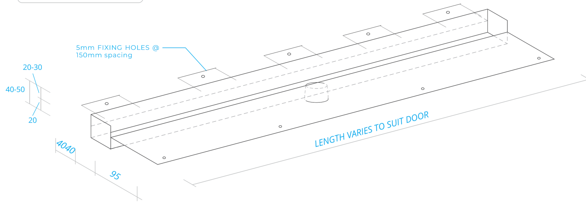
ISOMETRIC VIEW
