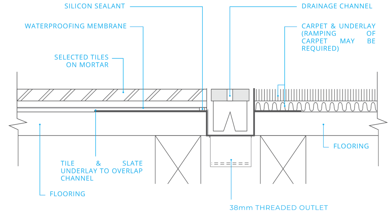
DETAIL VIEW
