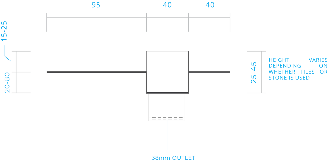
SECTION VIEW
