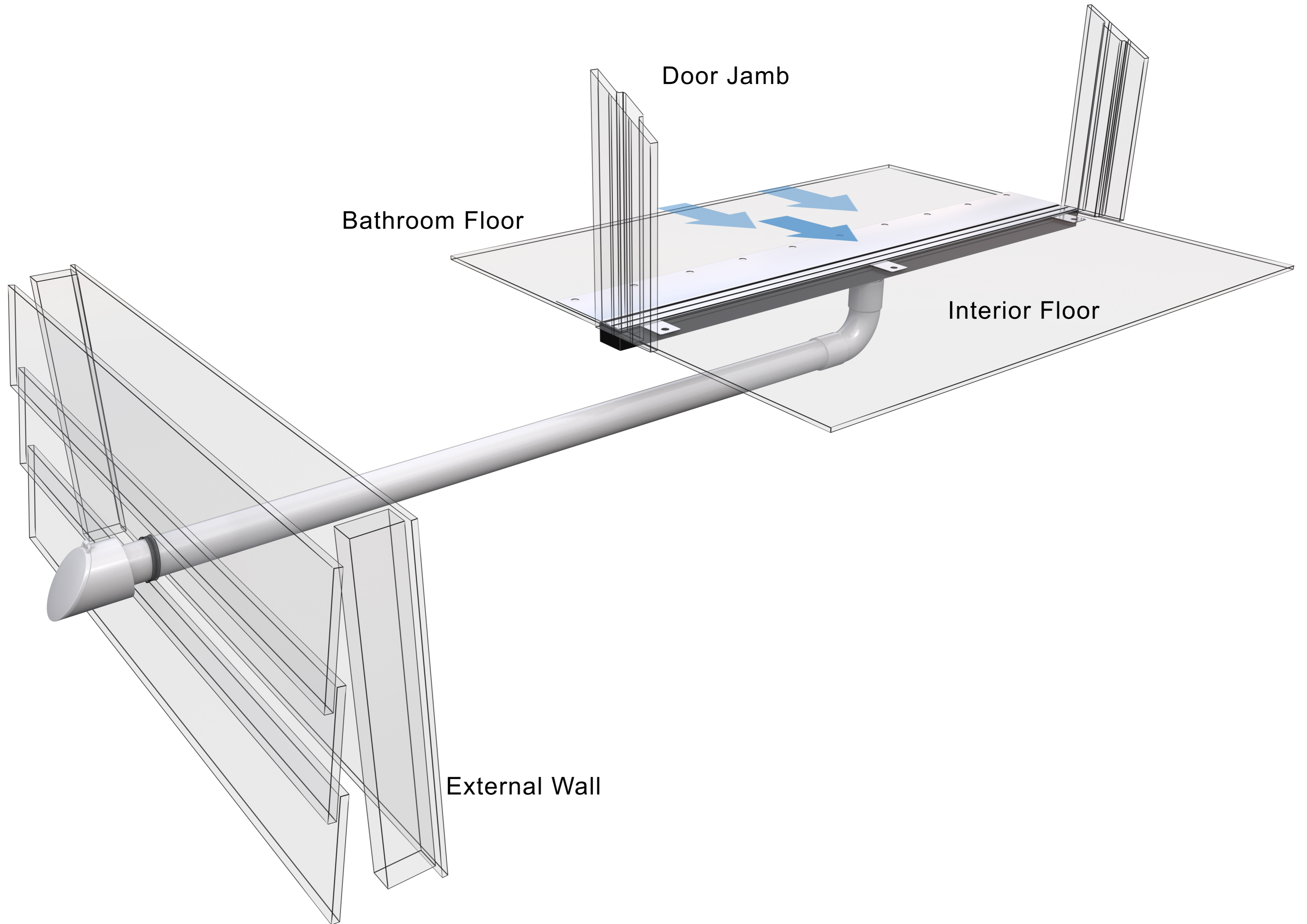
2 - 40mm Emergency Overflow Door Channel Plumbed Out Exterior Wall (Dry Waste)
