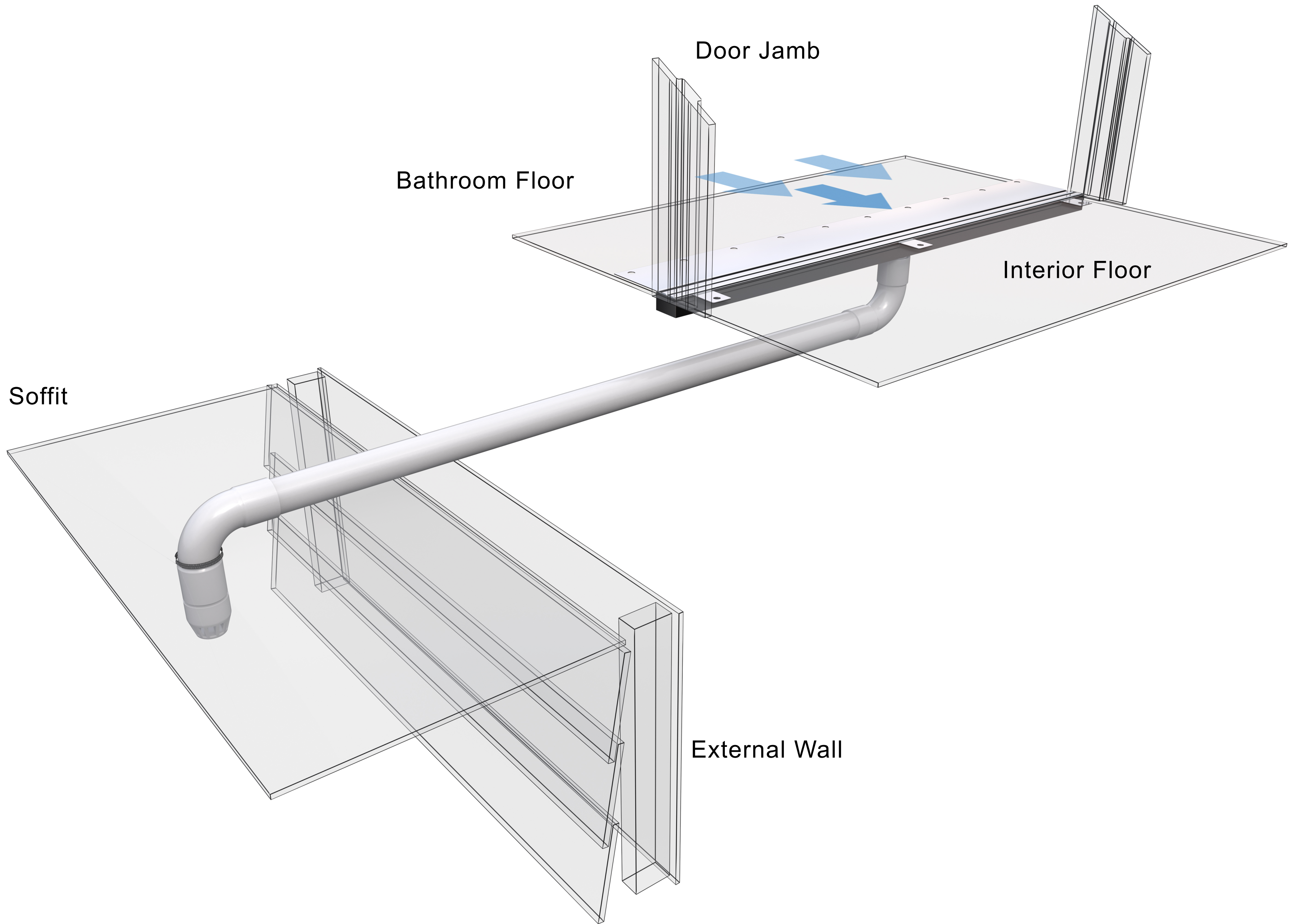
1 - 40mm Emergency Overflow Door Channel Plumbed Out Soffit (Dry Waste)
